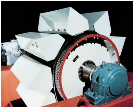
Drive drum of Belt Bucket Elevator type BWG
