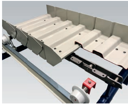
Pan Conveyor type KZB
